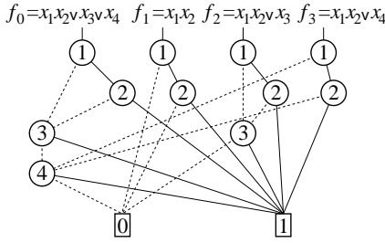
Fig. 3. Example of SBDD.
