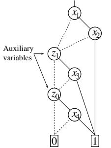
Fig. 6. BDD for ECFN considering variable ordering.
