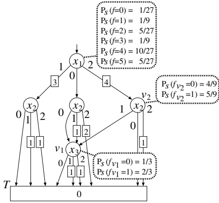
Figure 4. Analysis of the MSS using EVMDs [16].
